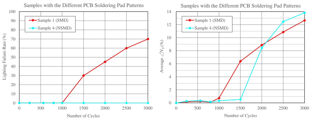
Figure 11. Lighting Failure Rate and Average \Delta V_F
