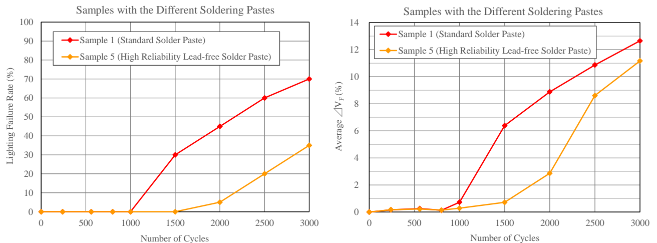
Figure 12. Lighting Failure Rate and Average \Delta V_F
