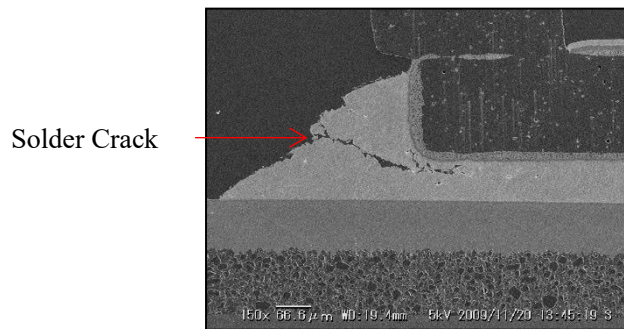
Figure 1. Example of a Solder Crack
