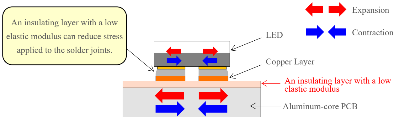
Figure 6. Aluminum-core PCB Containing an Insulating Layer with a Low Elastic Modulus
