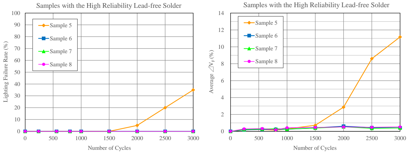
Figure 13. Lighting Failure Rate and Average \Delta V_F
